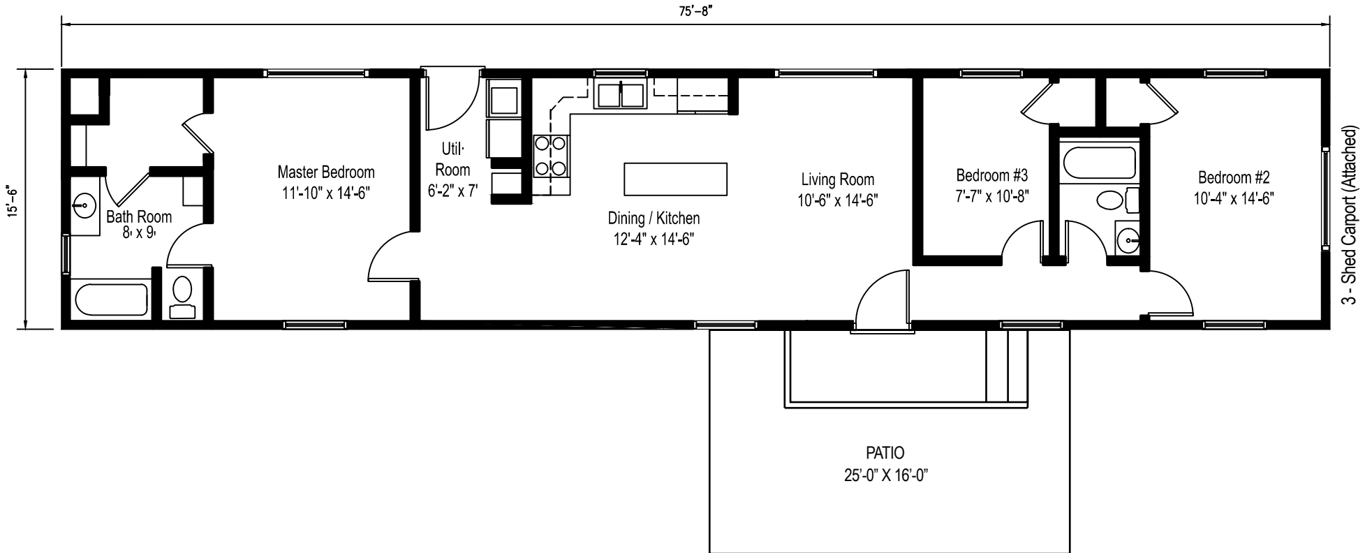
MOBILE HOME FLOOR PLAN
