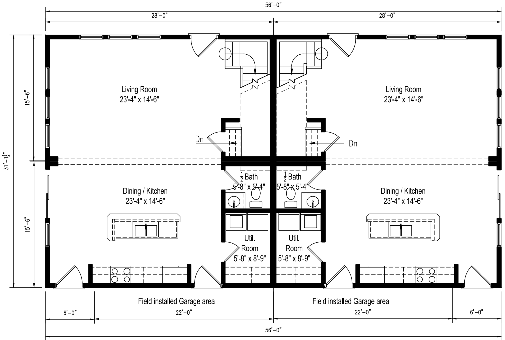
MULTI - FAMILY RESIDENCE 1ST FLOOR PLAN
