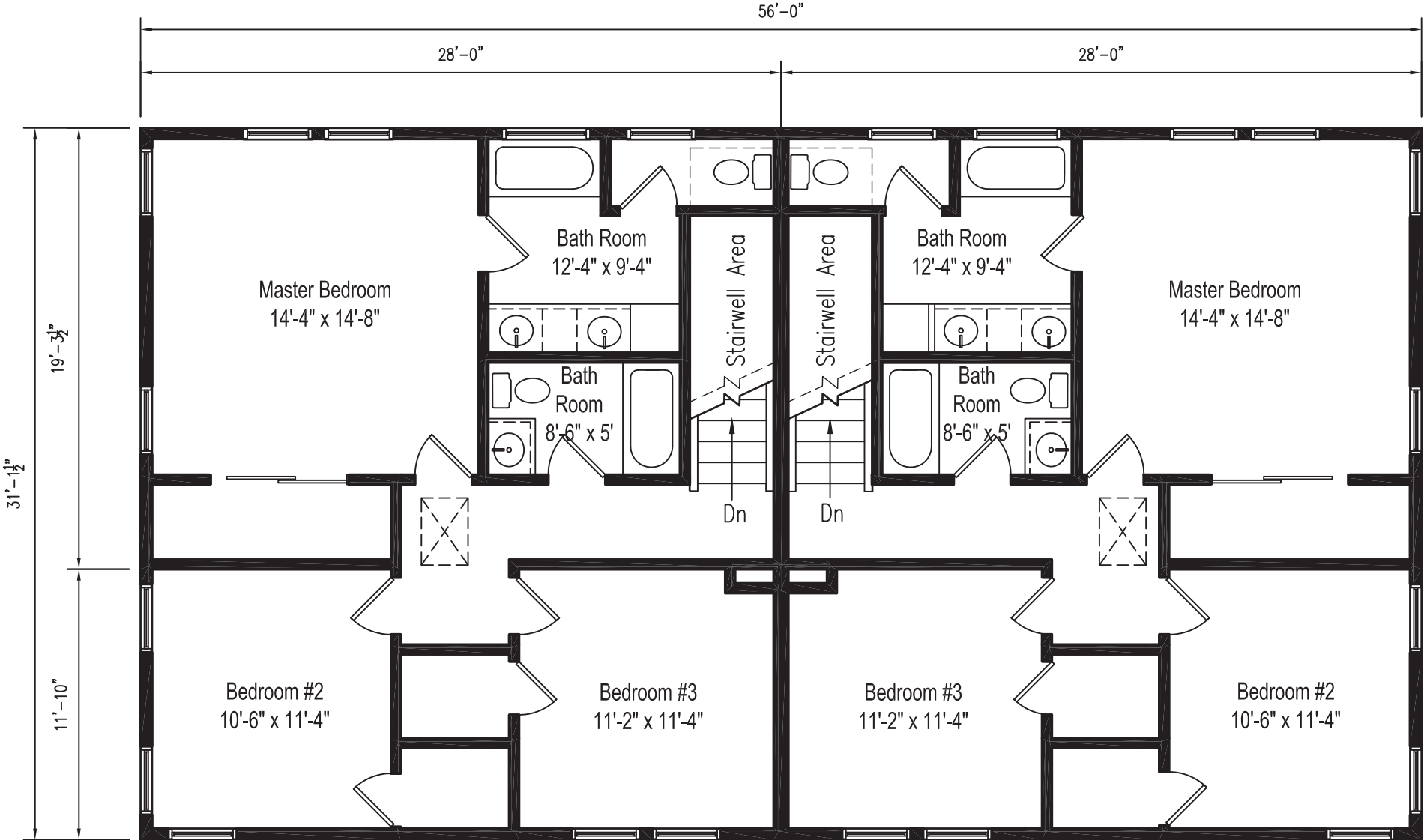
MULTI - FAMILY RESIDENCE 2ND FLOOR PLAN
