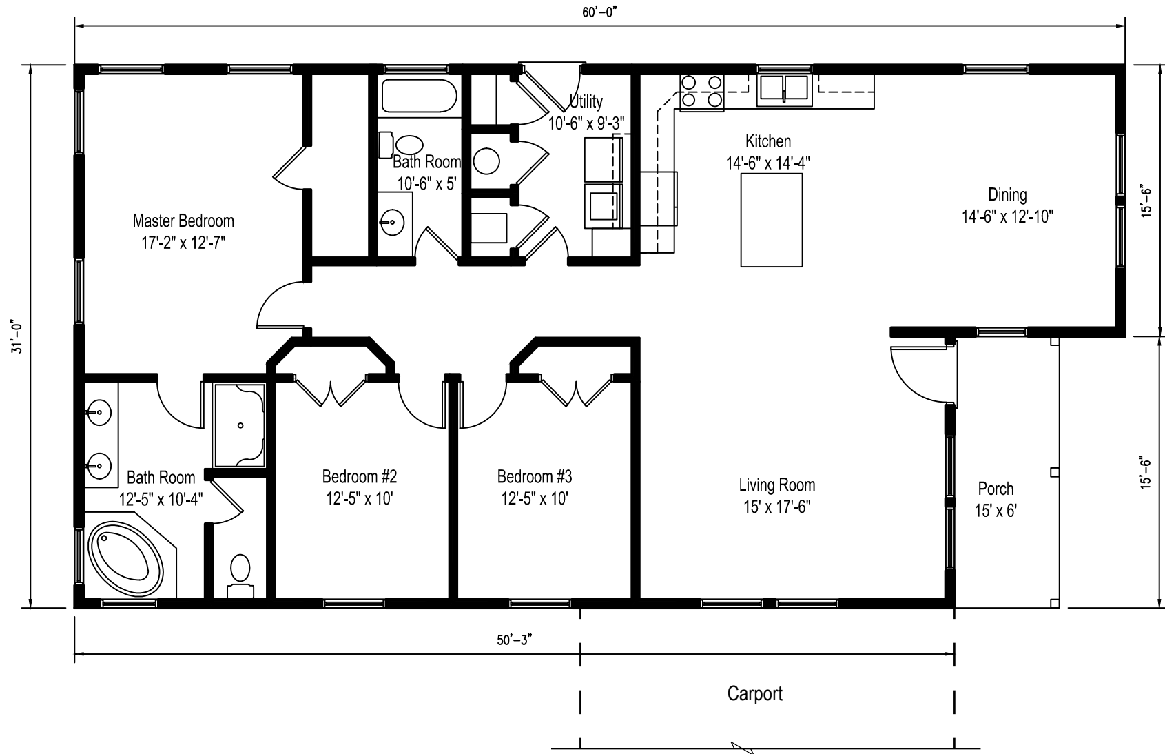
SINGLE FAMILY RESIDENCE (HALF - PORCH W/ CARPORT) FLOOR PLAN
